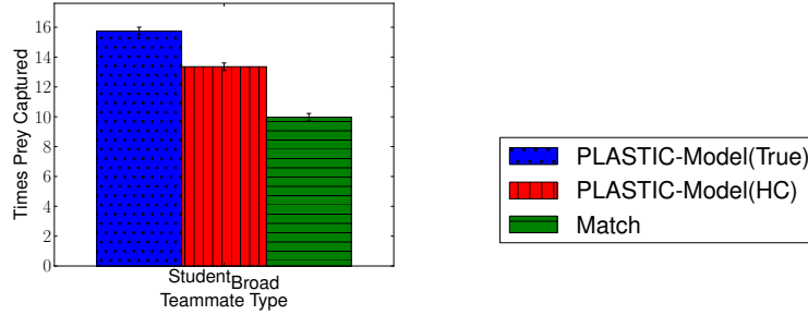
Figure 7.6: Results with unobserved externally-created teams (Student Broad ) on a 20x20 world.
