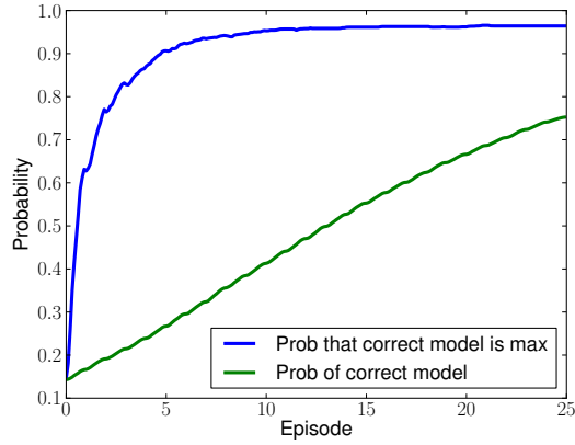
Figure 7.15: Belief of the probability of the correct model ( P(m^*|s, a) ) and probability of the correct model having the highest probability ( P(p^* = \max p_i|s, a) ) by PLASTIC-Policy in the full HFO task.
