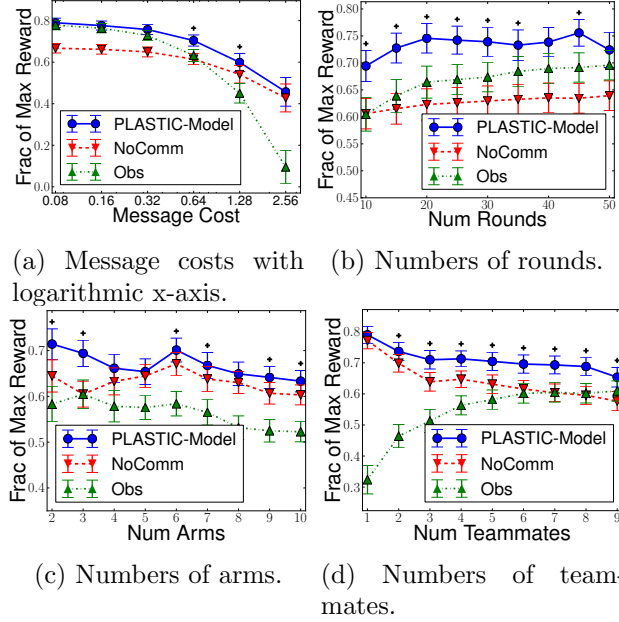
Figure 7.2: Normalized rewards with varied parameters when cooperating with externally-created teammates.
