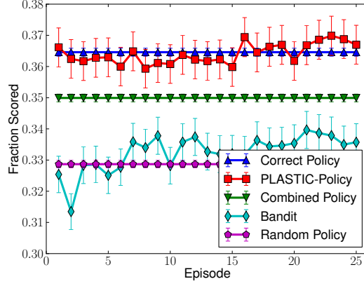
Figure 7.14: Scoring frequency in the full half field offense task.
