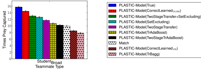
Figure 7.9: Comparing different transfer learning algorithms in PLASTIC-Model to improve results with ad hoc agents that have limited observations of their current teammates. Tests are in a 20x20 world with Student Broad teammates.
