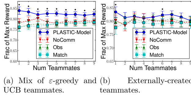
Figure 7.3: Normalized rewards when dealing with unknown arms and varying numbers of teammates.
