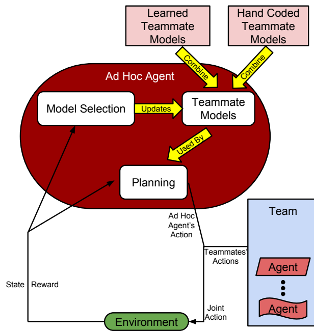
Figure 5.2: Overview of using the model-based approach of PLASTIC-Model to cooperate with unknown teammates.
