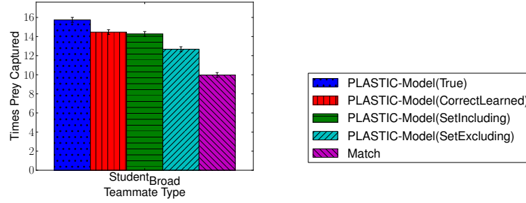
Figure 7.7: Results with PLASTIC-Model learning models of previously observed teammates when encountering teams from Student Broad on a 20x20 world.
