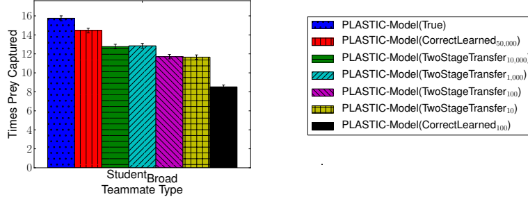
Figure 7.10: Evaluating PLASTIC-Model using TwoStageTransfer with varying amounts of target data. Tests are in a 20x20 world with Student Broad teammates.
