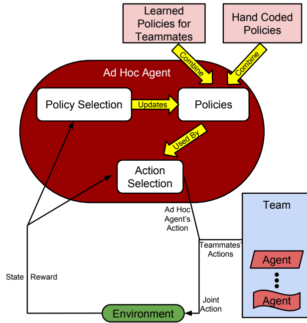
Figure 5.3: Overview of using the model-based approach of PLASTIC-Policy to cooperate with unknown teammates.
