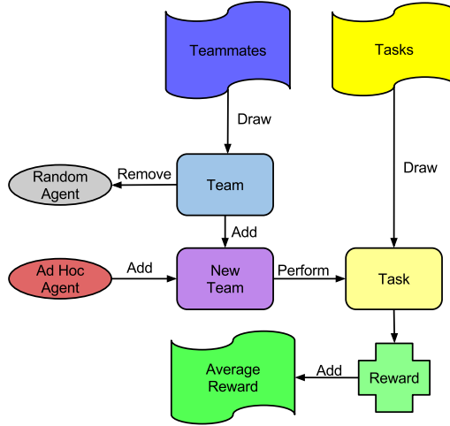
Figure 2.2: A visual representation of the evaluation algorithm given in Algorithm 1.
