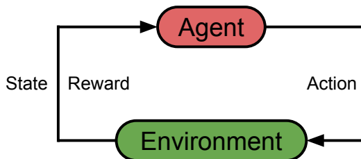
Figure 3.1: A single agent interacting with the environment in reinforcement learning
