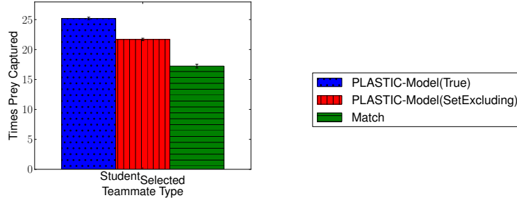
Figure 7.8: Results with PLASTIC-Model learning models of previously observed teammates when encountering teams from \text{Student}_{\text{Selected}} on a 20x20 world.
