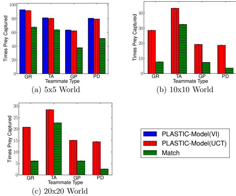
Figure 7.4: Results with known hand-coded teammates.
