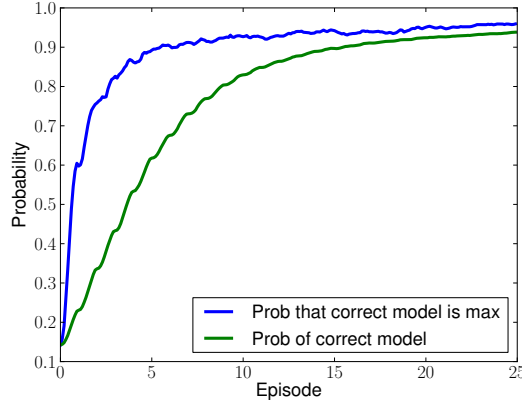
Figure 7.13: Belief of the probability of the correct model ( P(m^*|s, a) ) and probability of the correct model having the highest probability ( P(p^* = \max p_i|s, a) ) calculated by PLASTIC-Policy in the limited HFO task.
