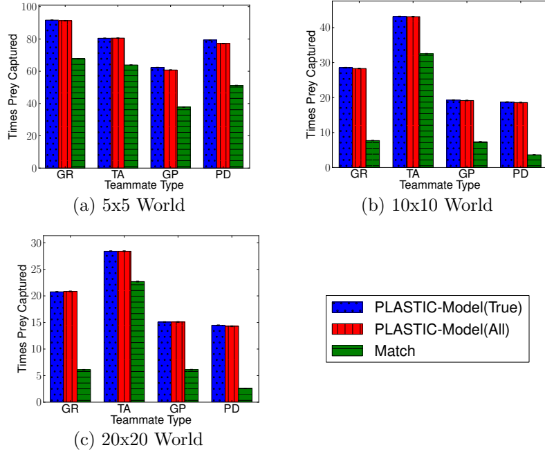
Figure 7.5: Results with unknown hand-coded teammates.
