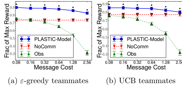
Figure 7.1: Normalized rewards with varied message costs with a logarithmic x-axis. Significance is denoted by “+”
