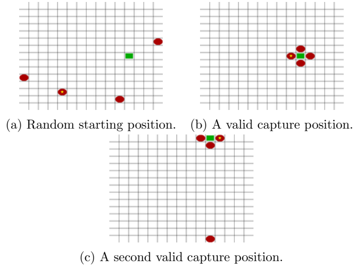
Figure 3.2: A view of the pursuit domain, where the rectangle is the prey, the ovals are predators, and the oval with the star is the ad hoc predator being evaluated.
