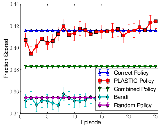
Figure 7.12: Scoring frequency in the limited half field offense task.
