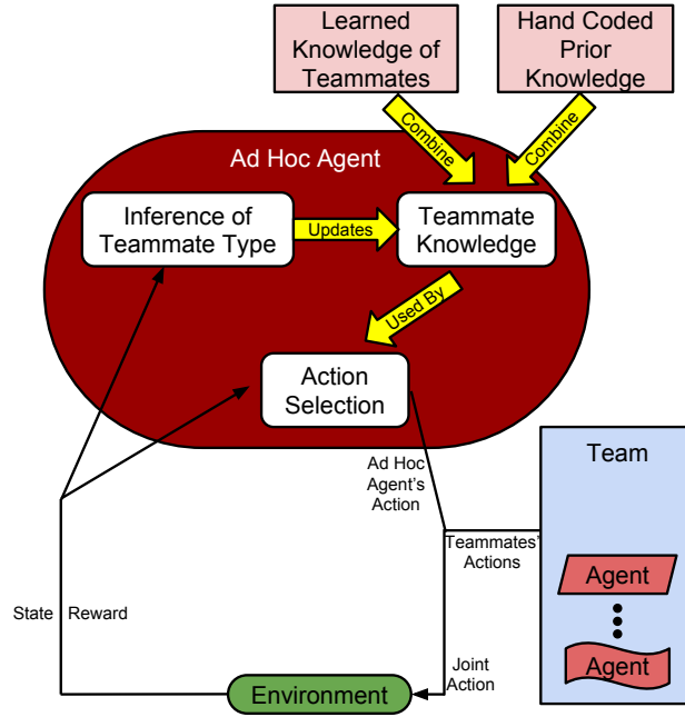
Figure 5.1: Overview of using PLASTIC to cooperate with unknown teammates.
